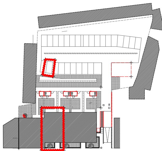
Inplantingsplan
